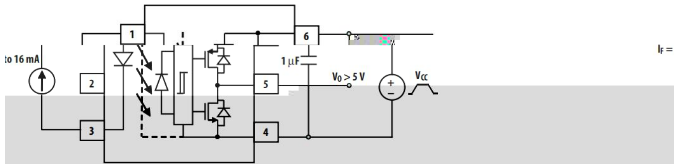
19. UVLO test circuit
