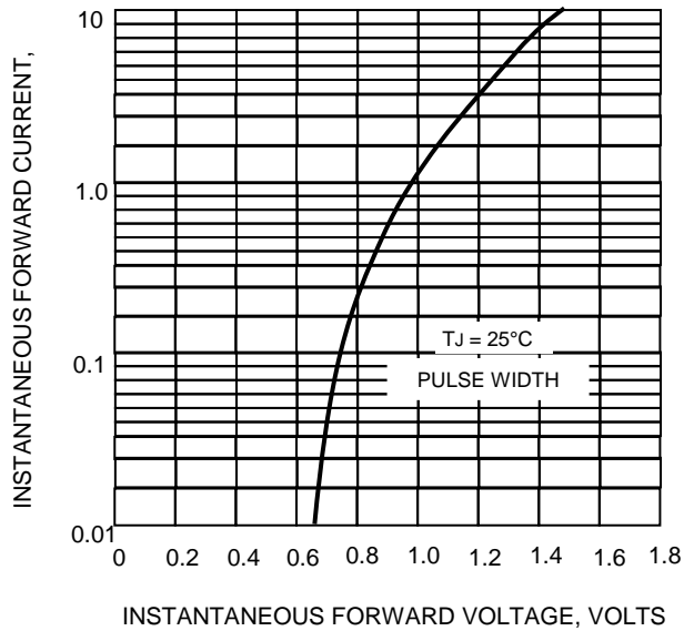
FIG.4-TYPICAL FORWARD CHARACTERISTICS
