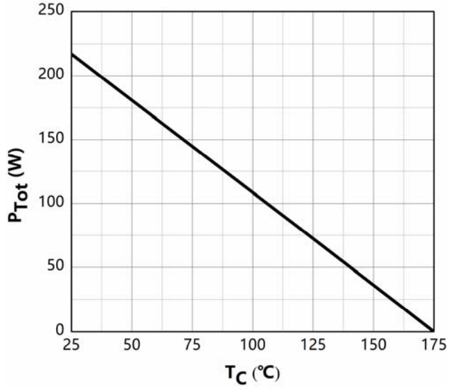
Figure 6. Power Derating
