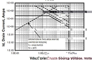
Figure 13. Maximum Safe Operating Area
